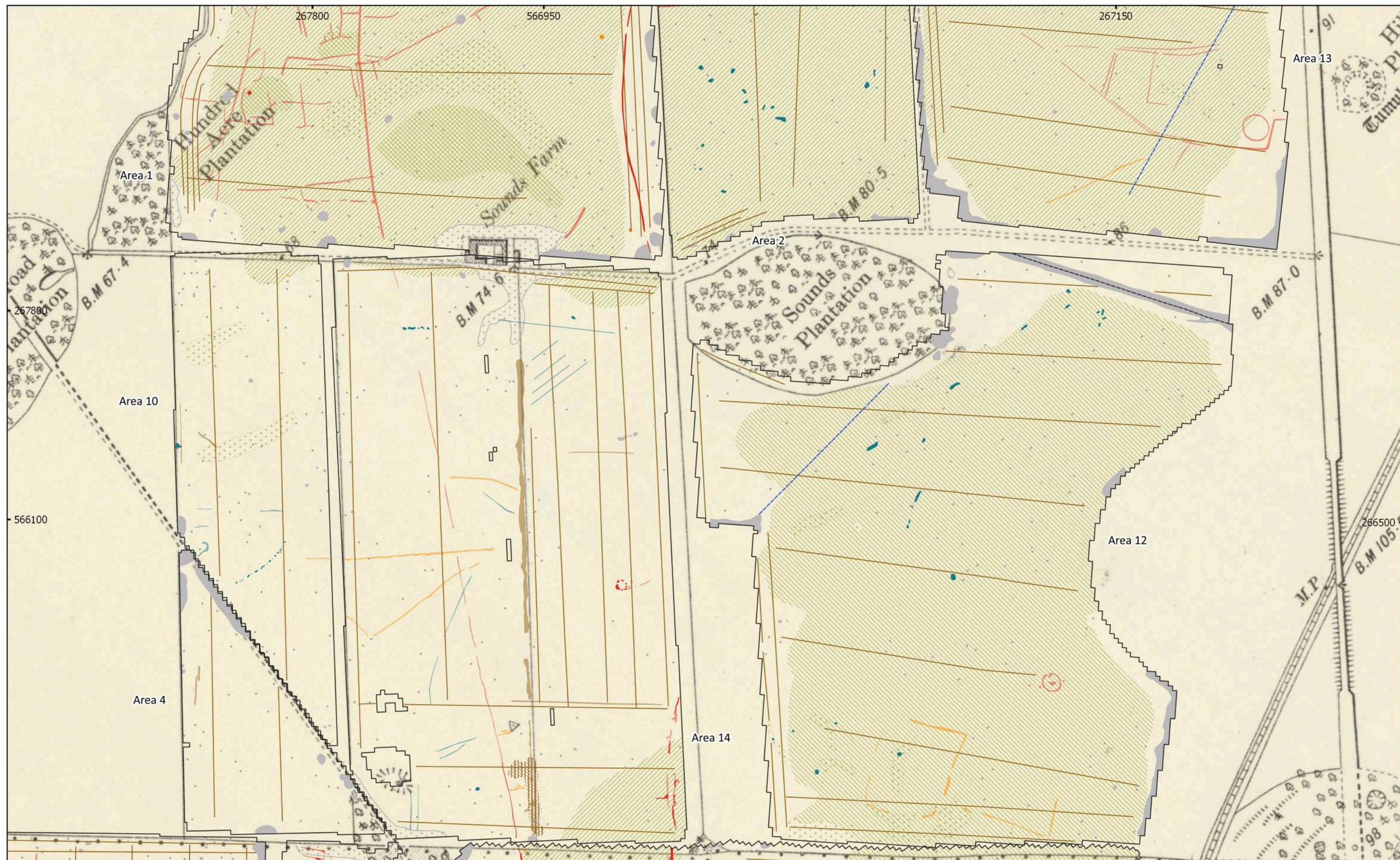
MSTL551 - Sunnica Energy Farm Reporting Zone F Figure F13 - Magnetic Interpretation Over Historic Maps (Southeast) 1:4,000 @ A3 Copyright Magnitude Surveys Ltd 2020 Contains historic maps: Ordnance Survey, 6" 2nd edition c. 1882-1913 © National Library of Scotland
